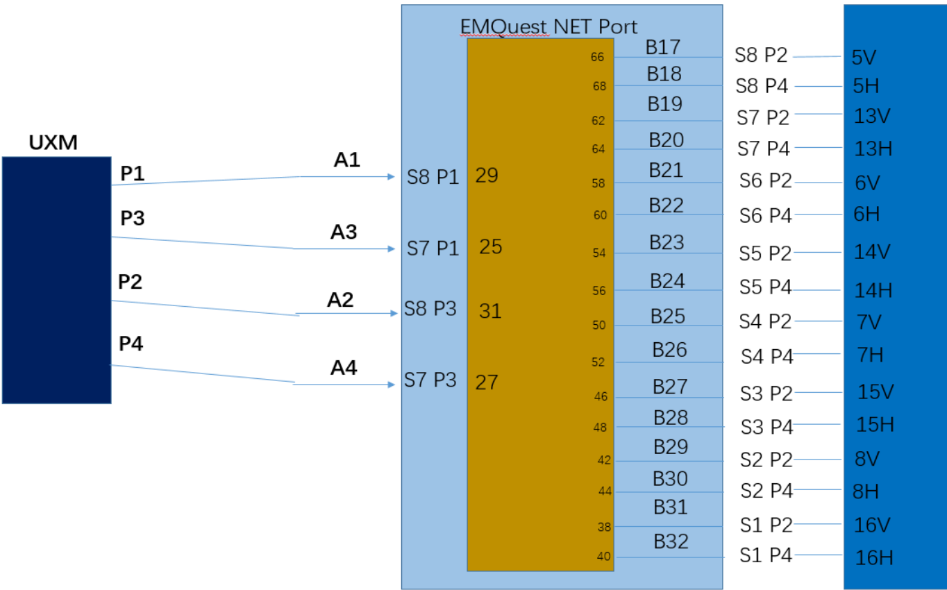
Vertex2 and AMP Probe Cabling Diagram 5G 16 probe
