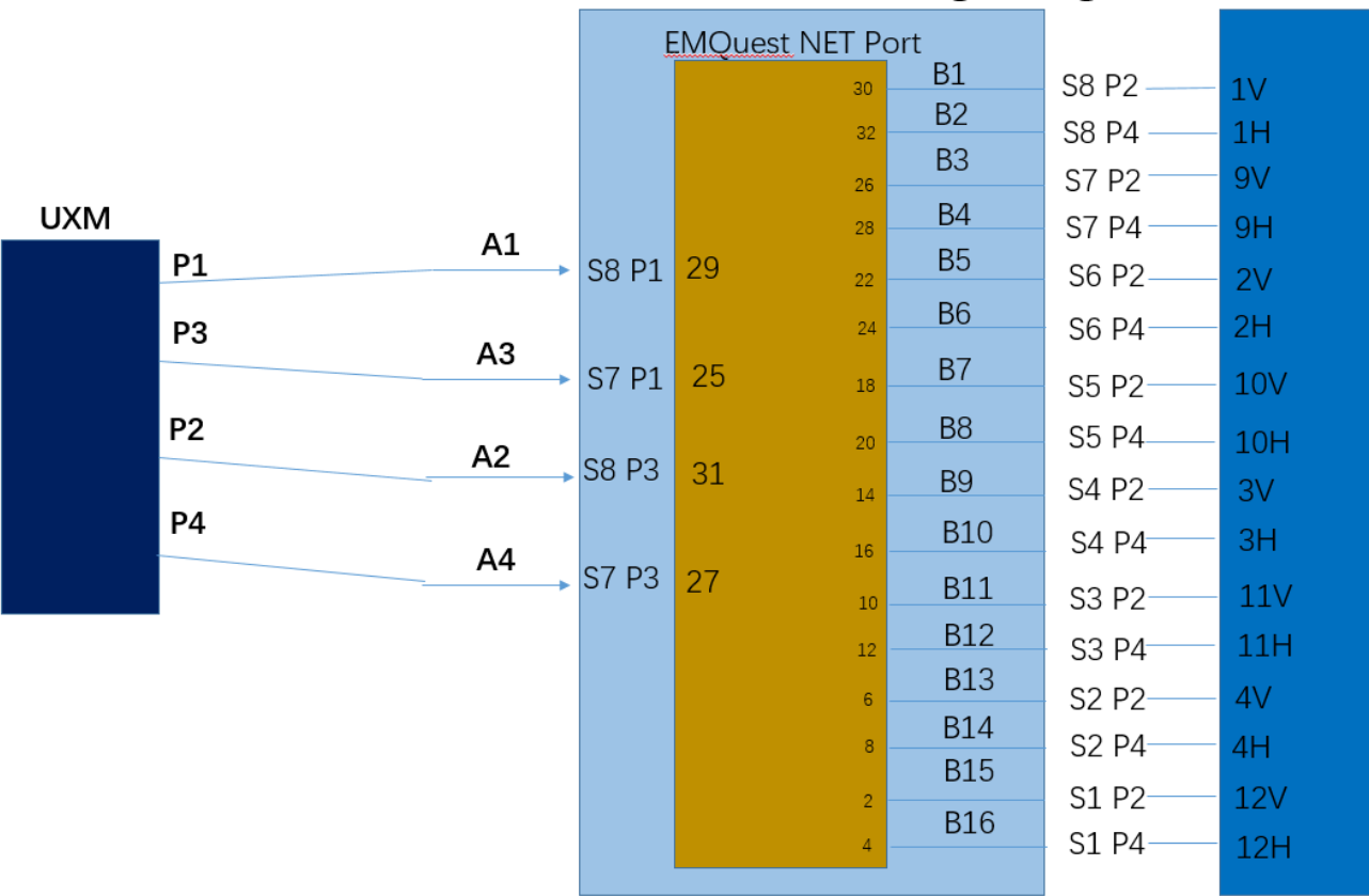
Vertex1 and AMP Probe Cabling Diagram 5G 16 probe
